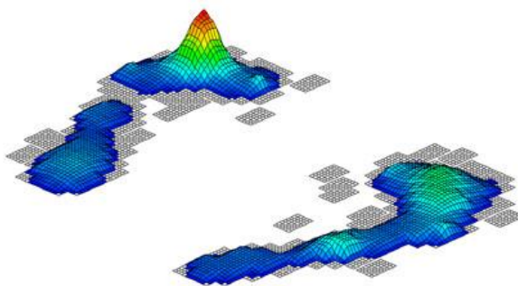
Fig 6. Results for static plantar measurements for left foot: max.124.74kPa; MT max.118.63 kPa min 3.96 kPa; heel max.19.8 kPa min.5.61kPa.
