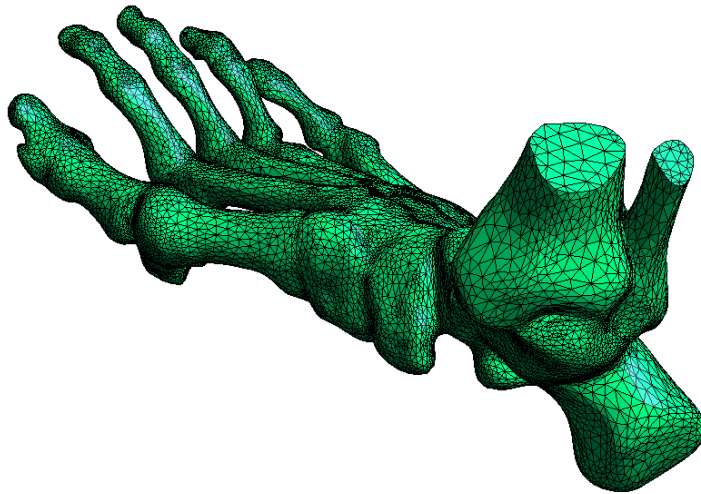
Fig. 3 3D finite element mesh of foot model after generation and smoothing techniques
