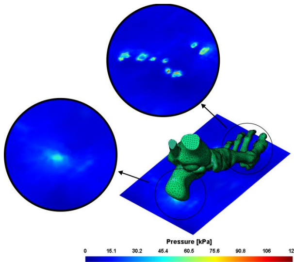
Fig 10. Effective stress distribution along plate for left foot
